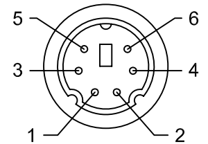
FRONT VIEW OF PLUG
